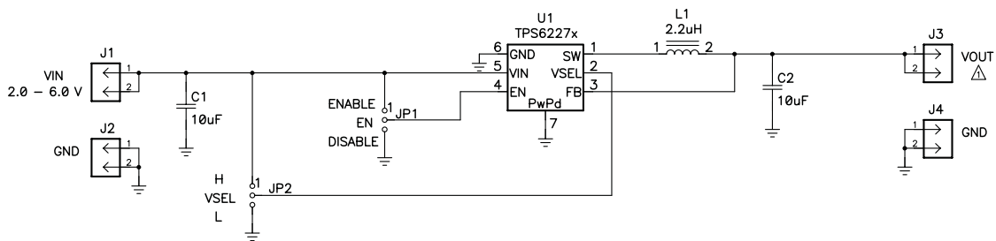
Figure 11. TPS6227XEVM-306 Schematic
