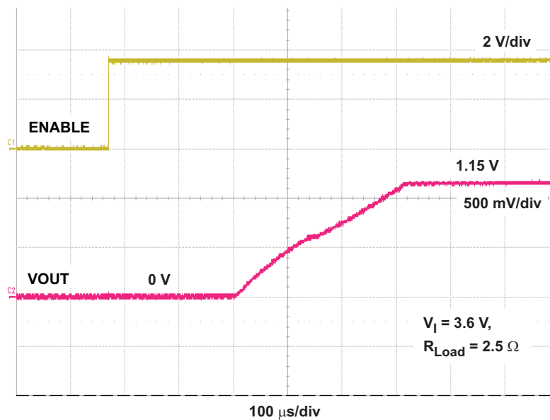
Figure 1. Start up from Enable, V_I = 3.6\text{ V} , V_{OUT} = 1.15\text{ V} , R_{Load} = 2.5\ \Omega
